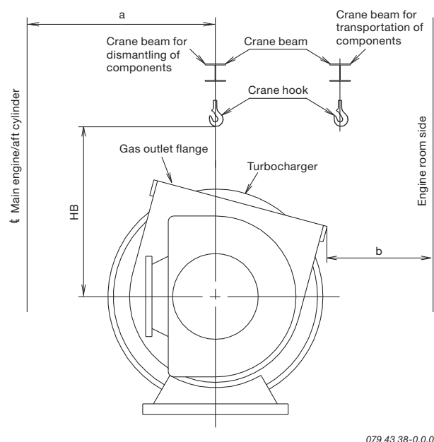
Fig. 5.03.01a: Required height and distance
