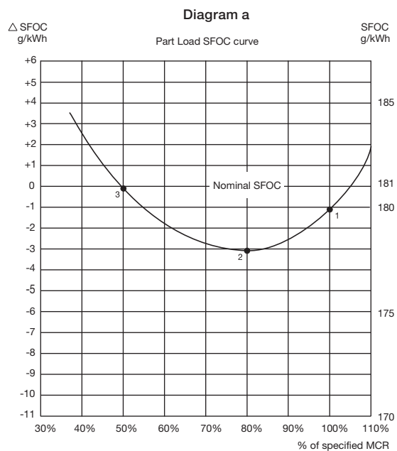
Fig. 2.10.01: Example of SFOC for derated 6S26MC6 with fixed pitch propeller and conventional turbocharger
