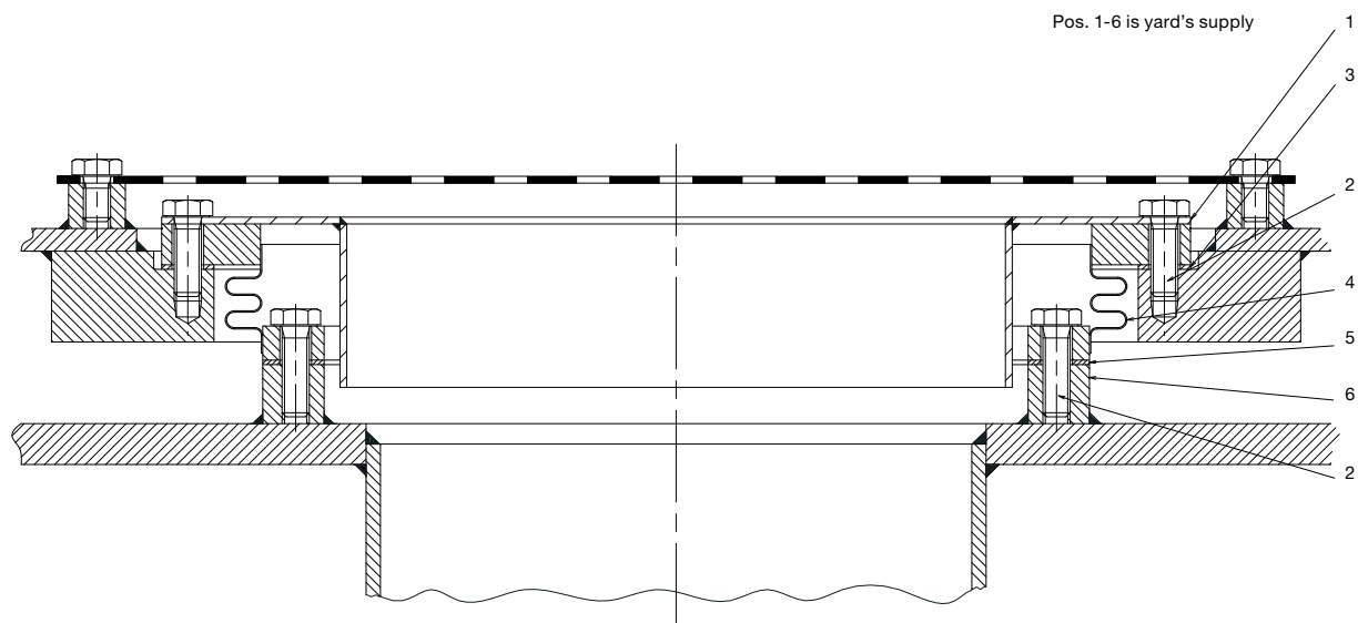
Fig. 8.05.01: Example of a lubricating oil outlet to bottom tank, S46MC-C/ME-B and S42MC is shown
