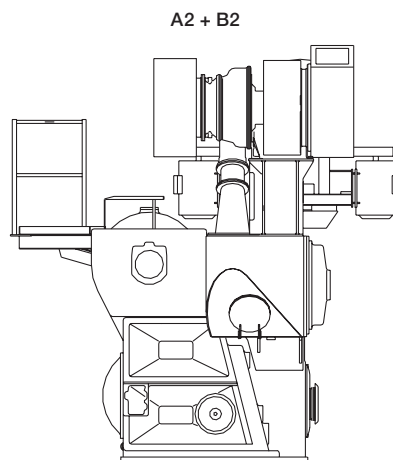
Top section
