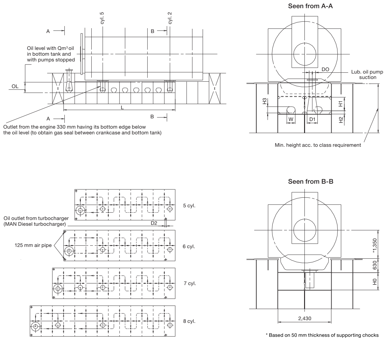
Fig. 8.06.01a: Lubricating oil tank, with cofferdam
