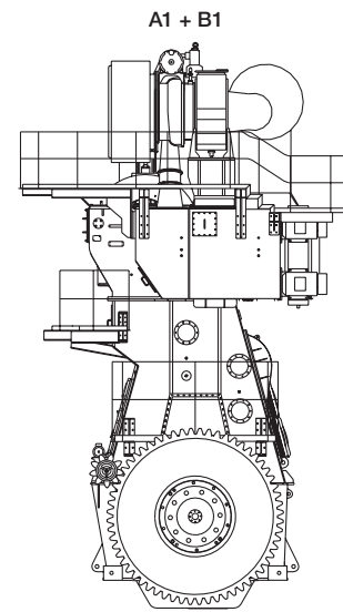
Engine complete
