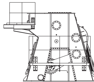
Frame box section
