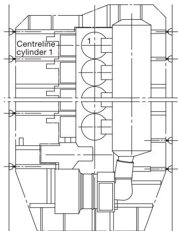
Fig. 5.14.01: Mechanical top bracing arrangement, aft end
