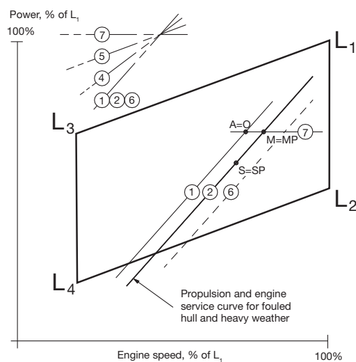
Layout diagram
