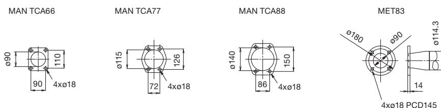
Fig. 5.10.01b: Connection E
