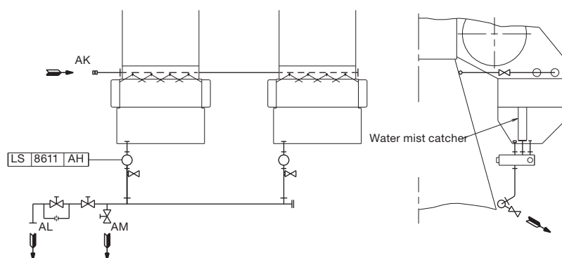
Fig. 14.05.01: Air cooler cleaning pipes
