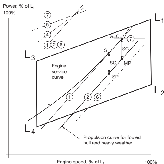
Layout diagram
