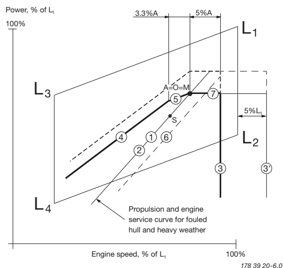
Load diagram
