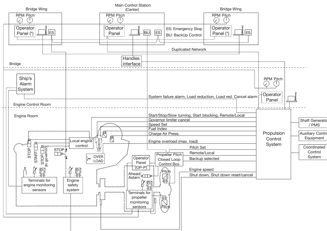
Fig. 5.18.07: Remote control system - Alphasonic 2000
