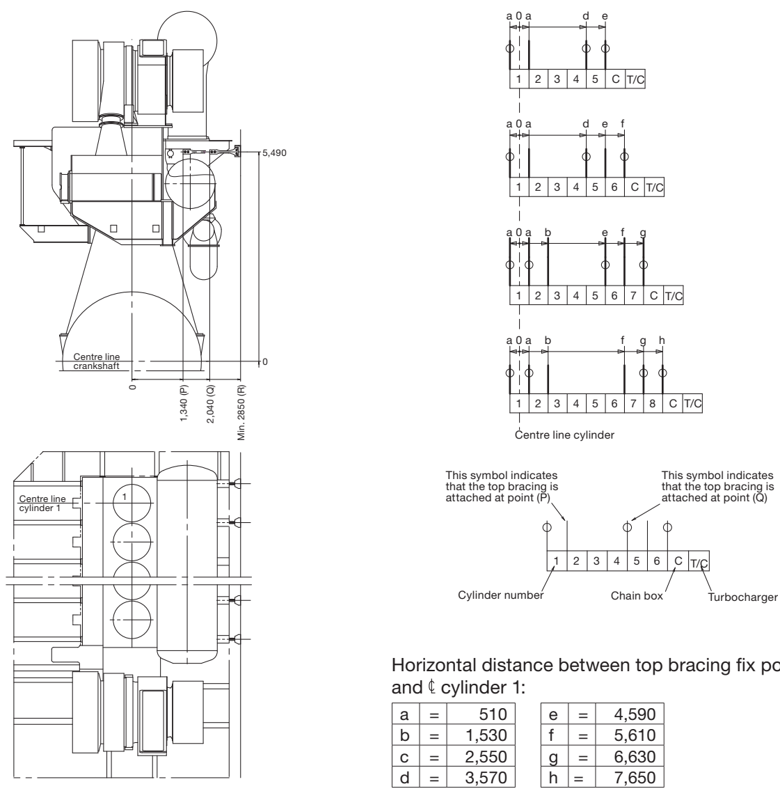
Fig. 5.14.01: Mechanical top bracing arrangement, aft end
