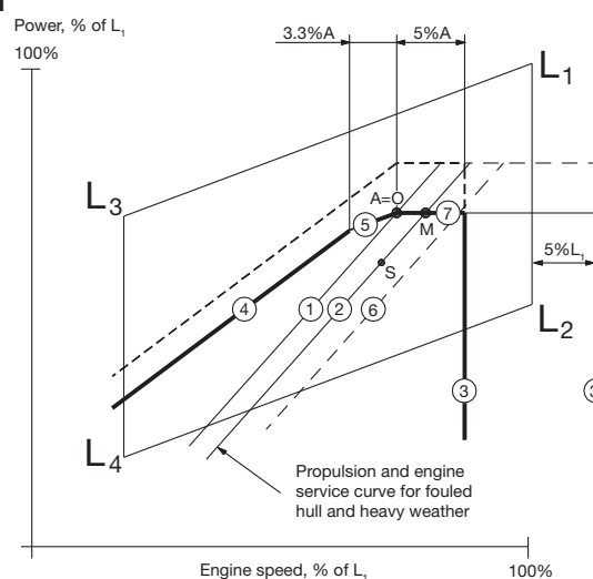
Load diagram
