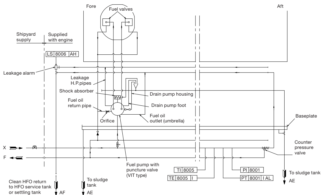
Fig. 7.03.01: Fuel oil and drain pipes, standard fuel pump
