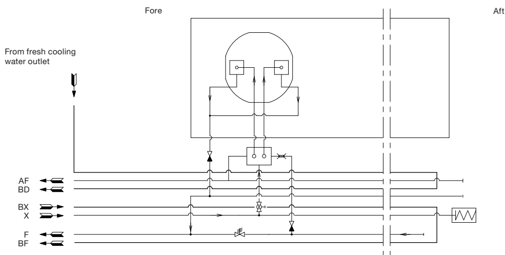
Fig. 7.04.03: Fuel oil pipe heat tracing
