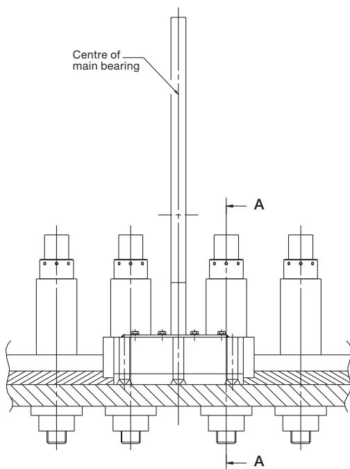
Fig. 5.12.02b: Profile of engine seating, end chocks, option: 4 82 620
