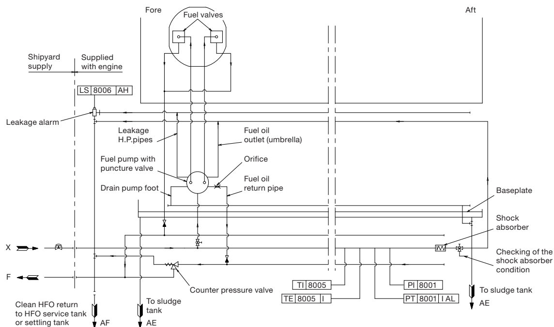
Fig. 7.03.01: Fuel oil and drain pipes, standard fuel pump
