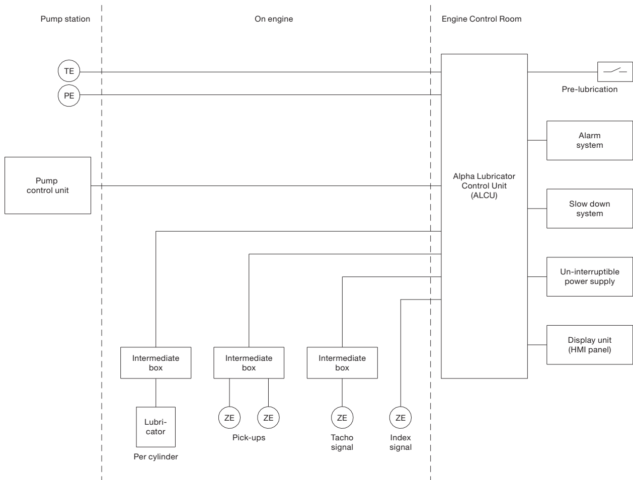
Fig. 9.02.05: Wiring diagram for MAN B&amp;W Alpha Cylinder Lubrication System, one lubricators per cylinder
