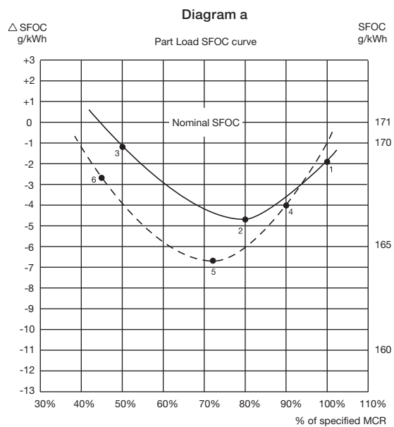
Fig. 2.10.01: Example of SFOC for derated S50MC-C7 with fixed pitch propeller and high efficiency turbocharger
