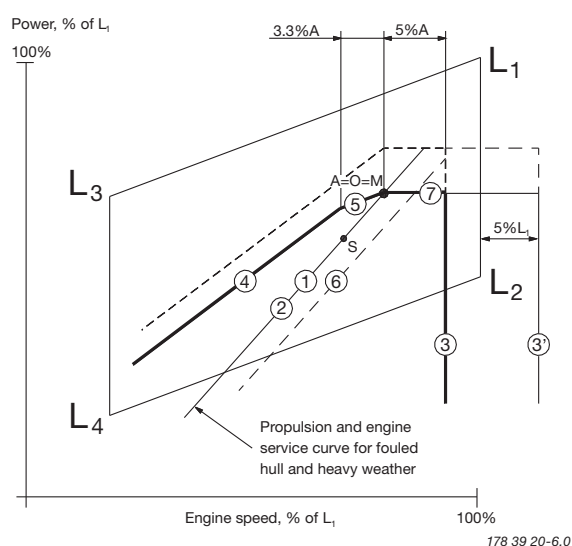
Load diagram
