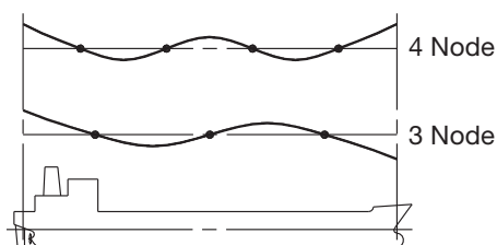
Fig. 17.03.02: Compensation of 2nd order vertical external moments
