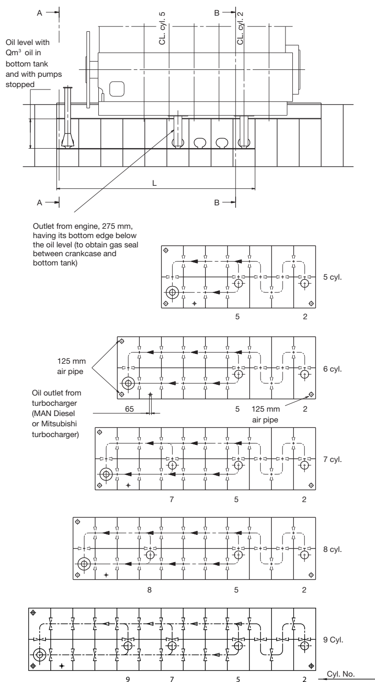
Fig. 8.06.01a: Lubricating oil tank, vertical outlet, with cofferdam
