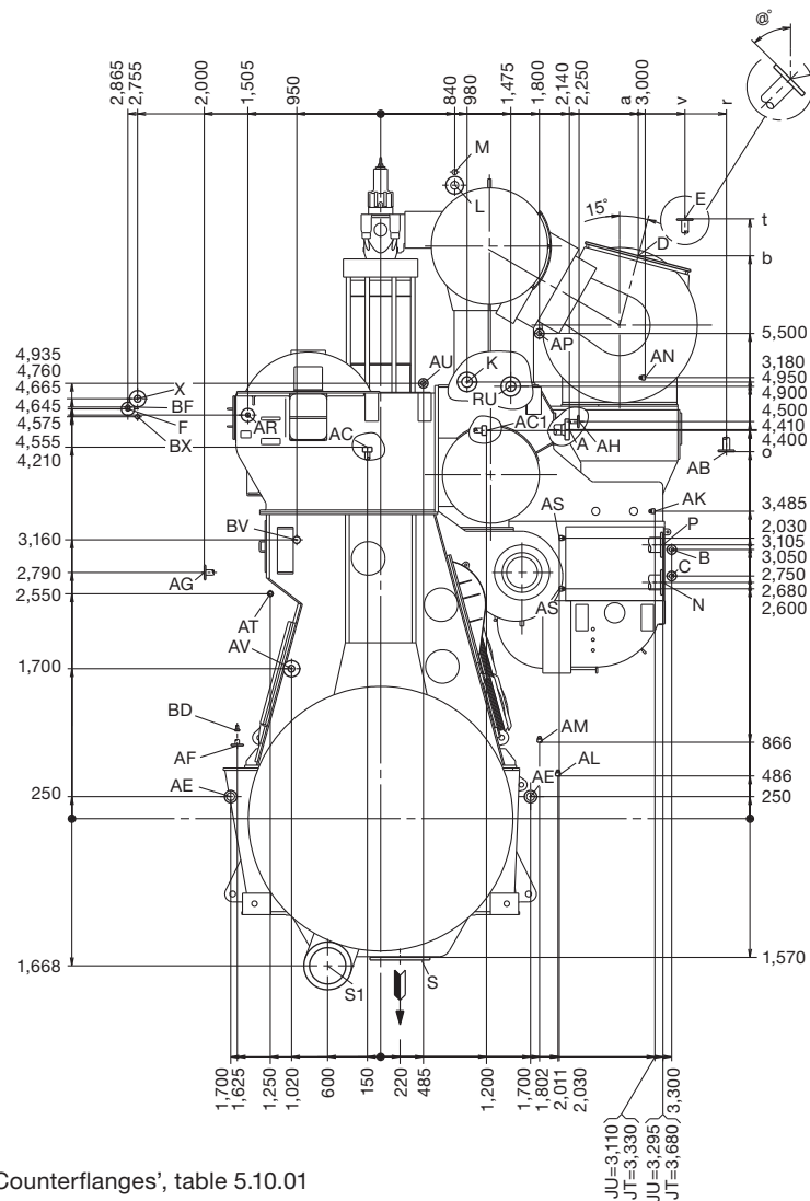
Fig. 5.09.02b: Engine pipe connections, 6S50MC-C7 with turbocharger on exhaust side
