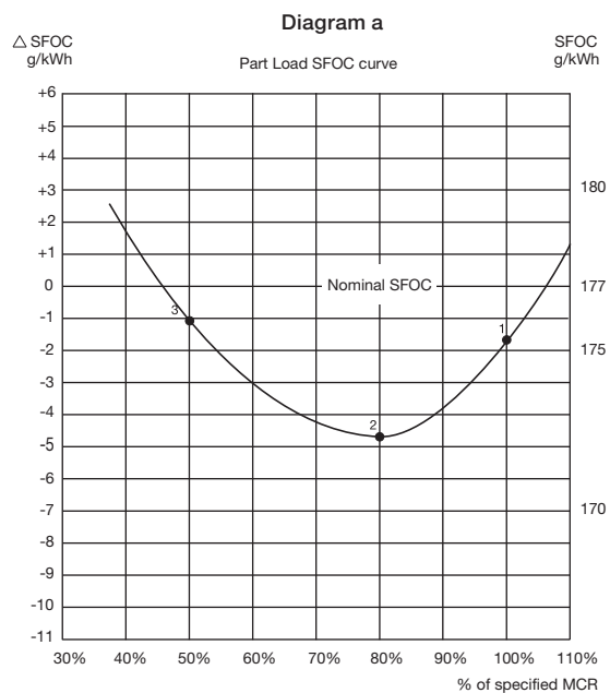
Fig. 2.10.01: Example of SFOC for derated 10K80MC-C6 with fixed pitch propeller and high efficiency turbocharger
