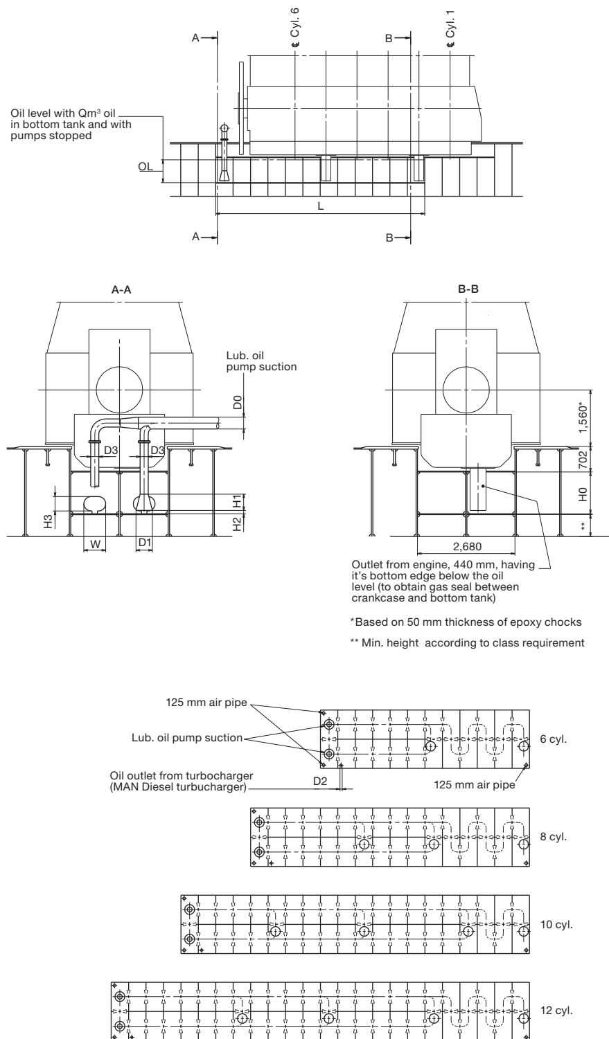
Fig. 8.06.01a: Lubricating oil tank, with cofferdam
