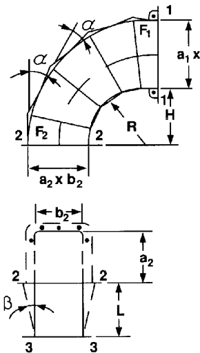
Intake Elbow Flange
