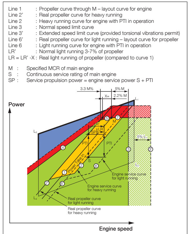
Fig. 23b: Example 4 with FPP – engine load diagram with PTI and extended speed limit
