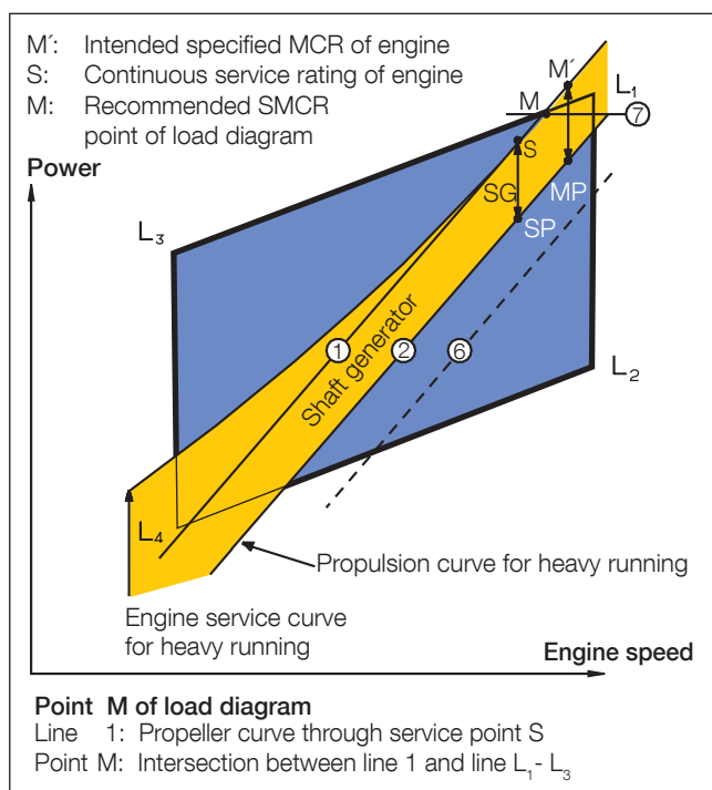
Fig. 22a: Example 3 with FPP – engine layout with SG (special case)
