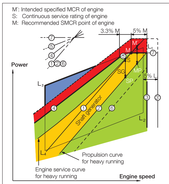
Fig. 22b: Example 3 with FPP – engine load diagram with SG (special case)
