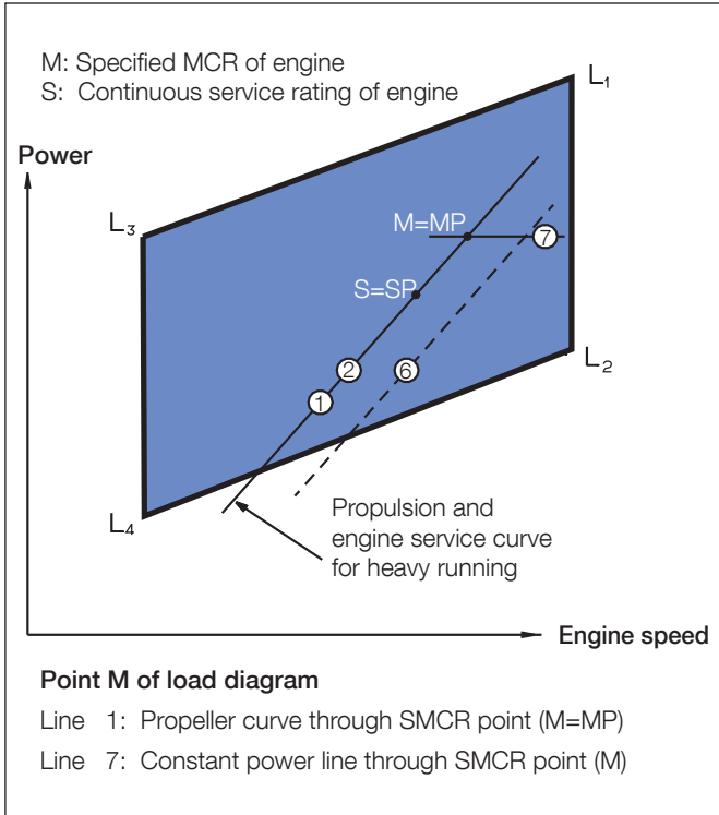
Fig. 20a: Example 1 with FPP – engine layout without SG (normal case)
