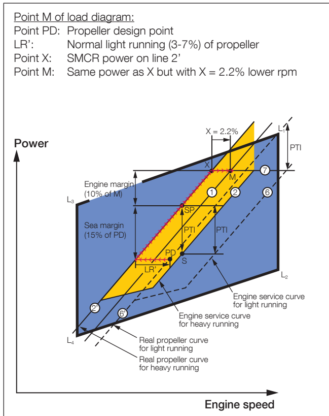
Fig. 23a: Example 4 with FPP – engine layout with PTI and extended speed limit
