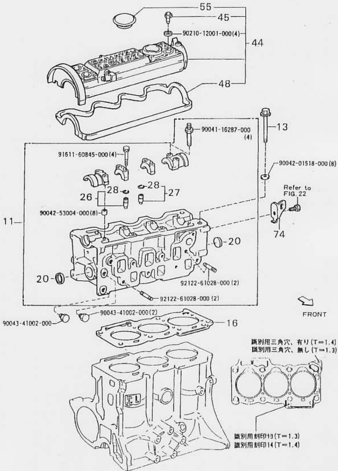
FIG. 6 CYLINDER HEAD
