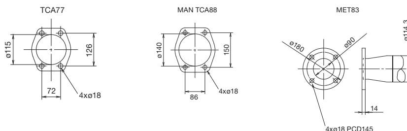
Fig. 5.10.01b: Connection E
