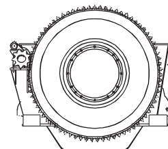
Bedplate/crankshaft section
