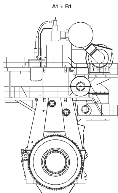
Engine complete
