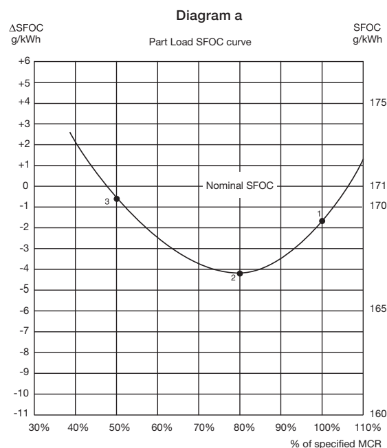
Fig. 2.10.01: Example of SFOC for derated S80MC-C8 with fixed pitch propeller and high efficiency turbocharger
