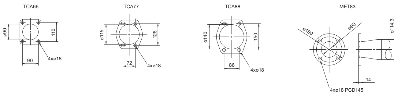
Fig. 5.10.01b: Connection E
