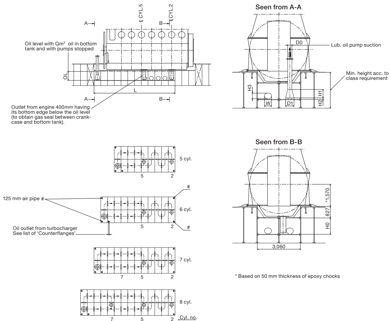
Fig. 8.06.01a: Lubricating oil tank, with cofferdam
