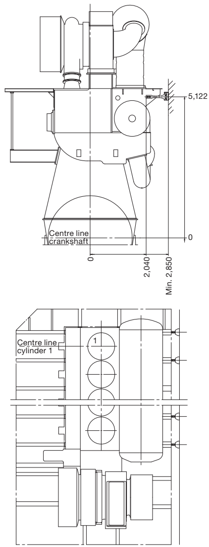
Fig. 5.14.01: Mechanical top bracing arrangement, aft end
