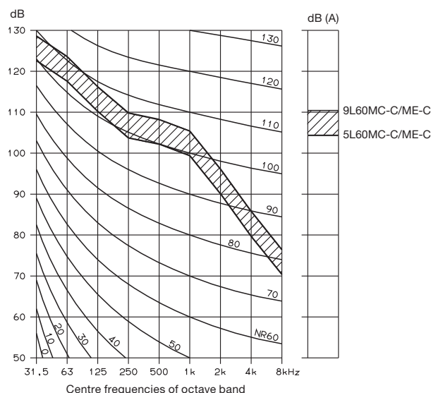
Fig. 15.04.02: ISO's NR curves and typical sound pressure levels from the engine's exhaust gas system. The noise levels at nominal MCR and a distance of 1 metre from the edge of the exhaust gas pipe opening at an angle of 30 degrees to the gas flow and valid for an exhaust gas system – without boiler and silencer, etc. Data for a specific engine and cylinder no. is available on request.
