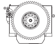
Bedplate/crankshaft section
